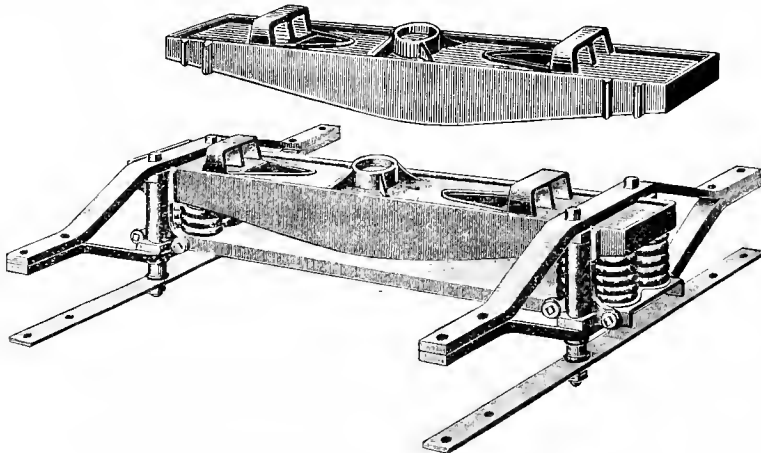
Figs. 4790-91. THE AMERICAN STEEL TRUCK-BOLSTER. THE AMERICAN STEEL CASTING COMPANY.
